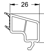
Glasleiste 26/25 Glazing bead 26/25 19559...
