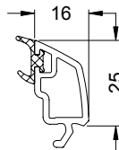
Glasleiste 16/25 Glazing bead 16/25 19584...
