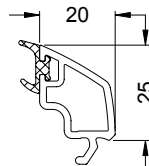
Glasleiste 20/25 Glazing bead 20/25 19586...
