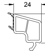
Glasleiste 24/25 Glazing bead 24/25 19558...
