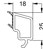
Glasleiste 18/25 Glazing bead 18/25 19555...
