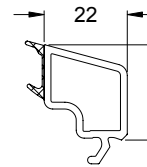
Glasleiste 22/25 Glazing bead 22/25 19557...
